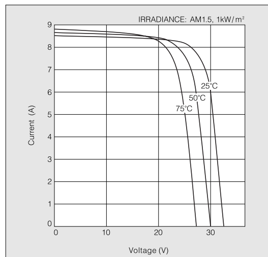
Current-Voltage characteristics of Photovoltaic Module KD210GH-2P at various cell temperatures
