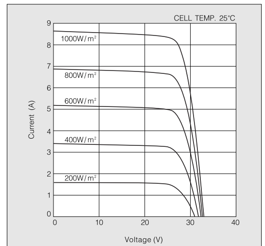
Current-Voltage characteristics of Photovoltaic Module KD210GH-2P at various irradiance levels
